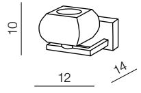
Rubic 1 wall AZ0488 G9 1x 40W metal/chrome/acryl
