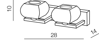
Rubic 2 wall AZ0491 G9 2x 40W metal/chrome/acryl
